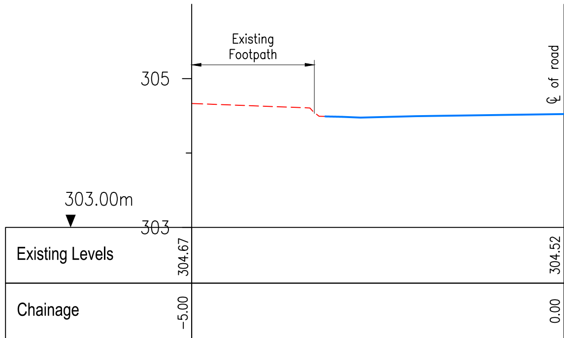
SECTION 1 - Ch-3 Scale 1:50
