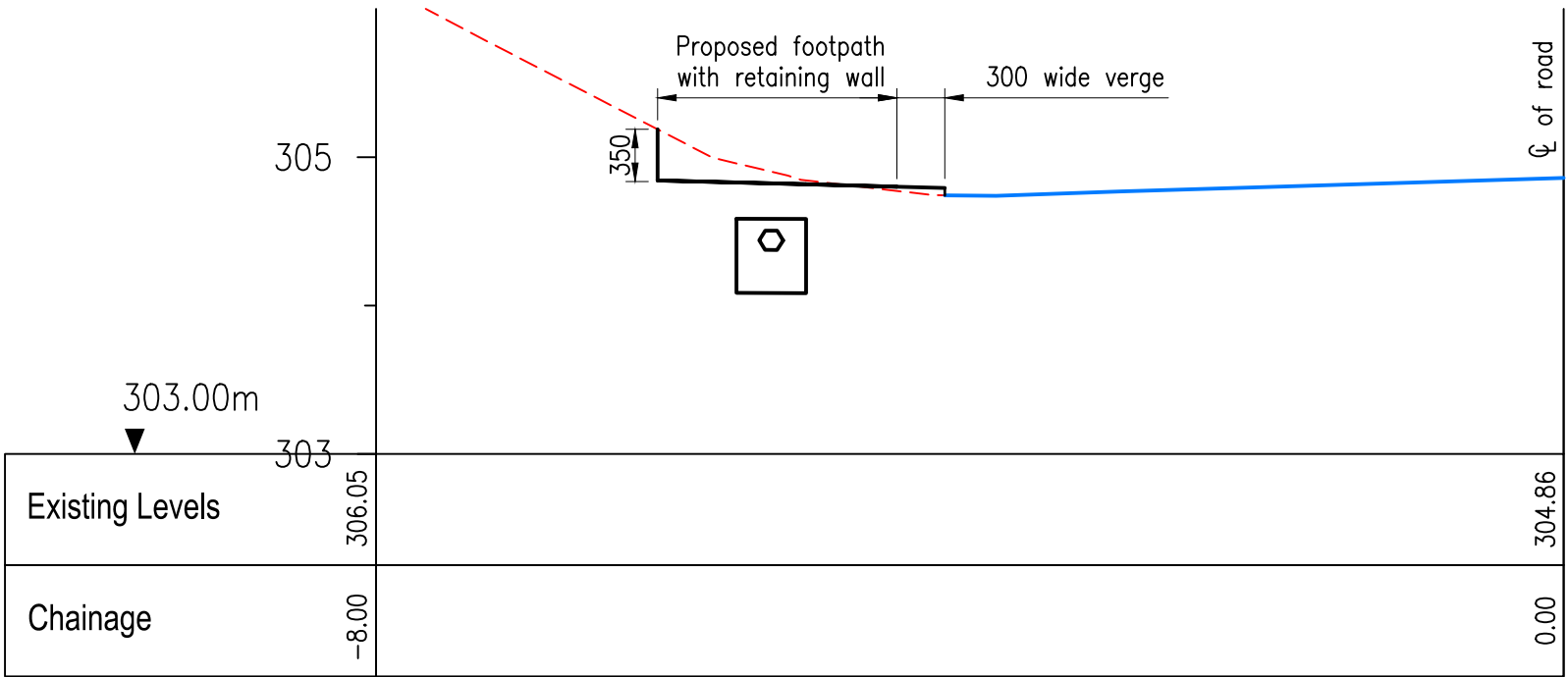
SECTION 7 - Ch109 Scale 1:50
