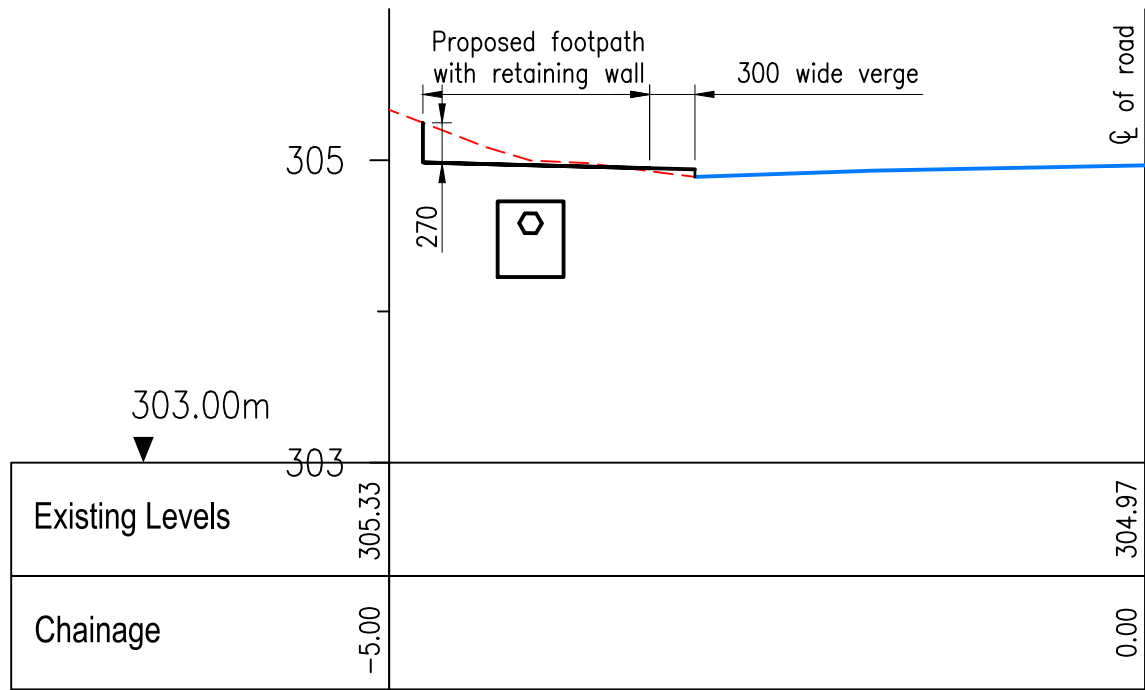
SECTION 5 - Ch53 Scale 1:50
