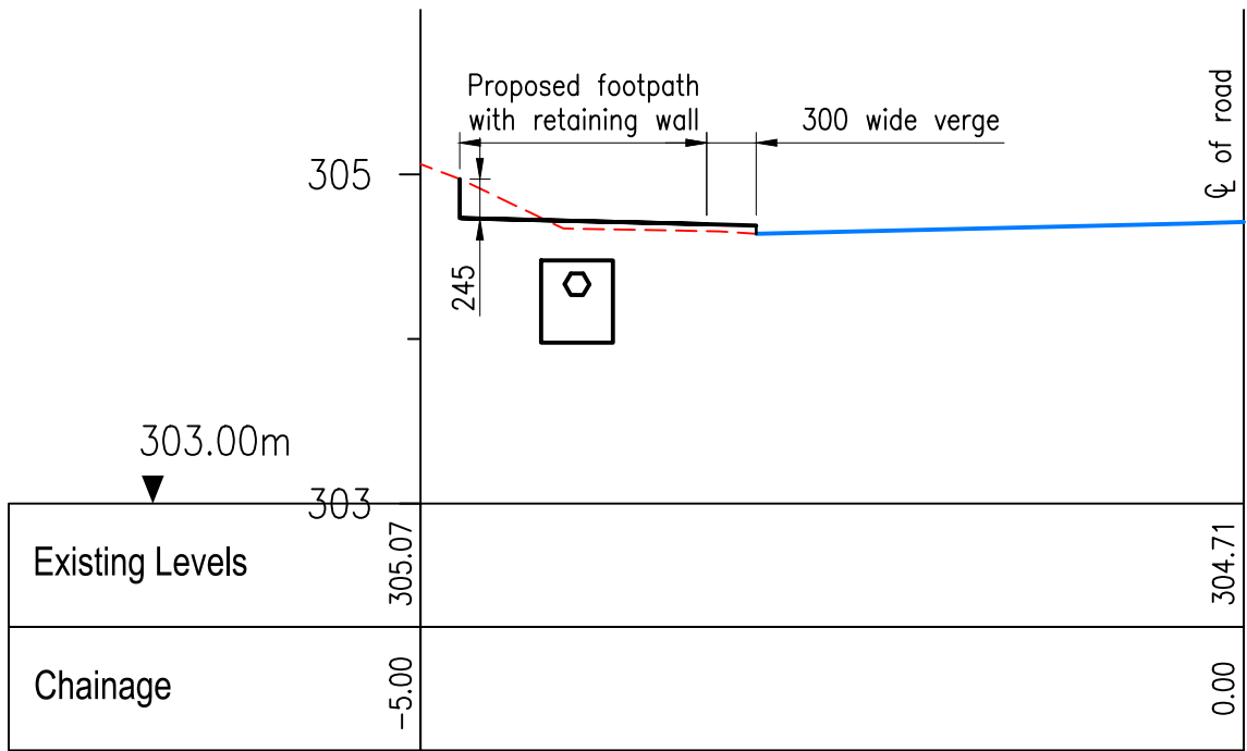
SECTION 8 - Ch137 Scale 1:50
