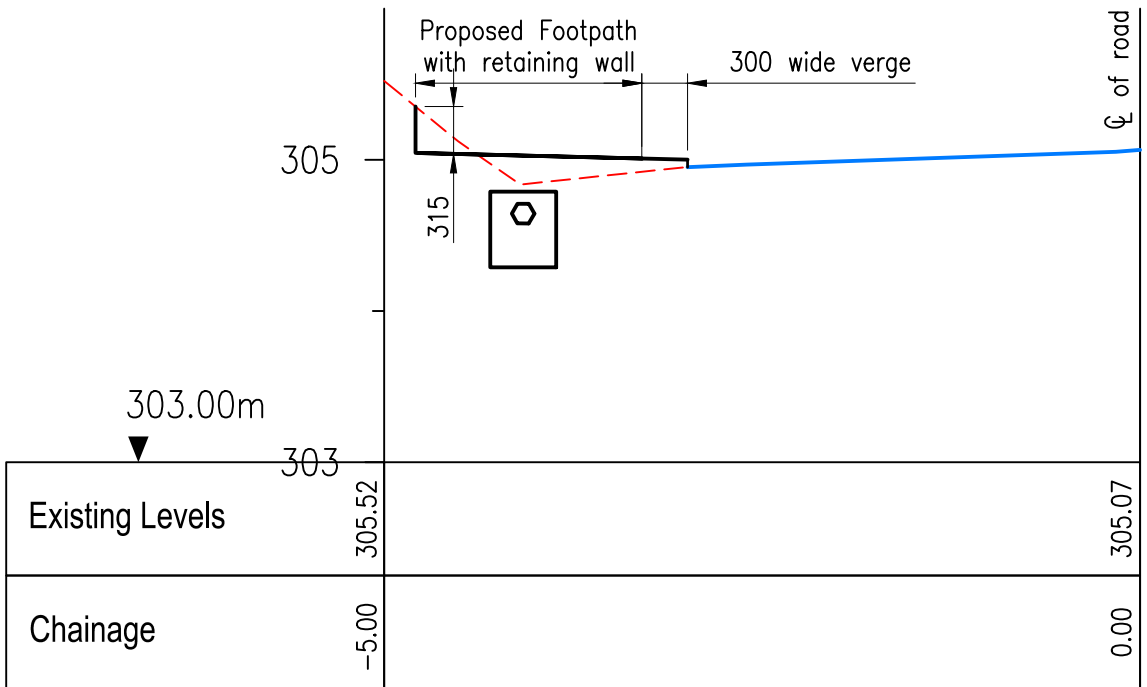
SECTION 2 - Ch17 Scale 1:50
