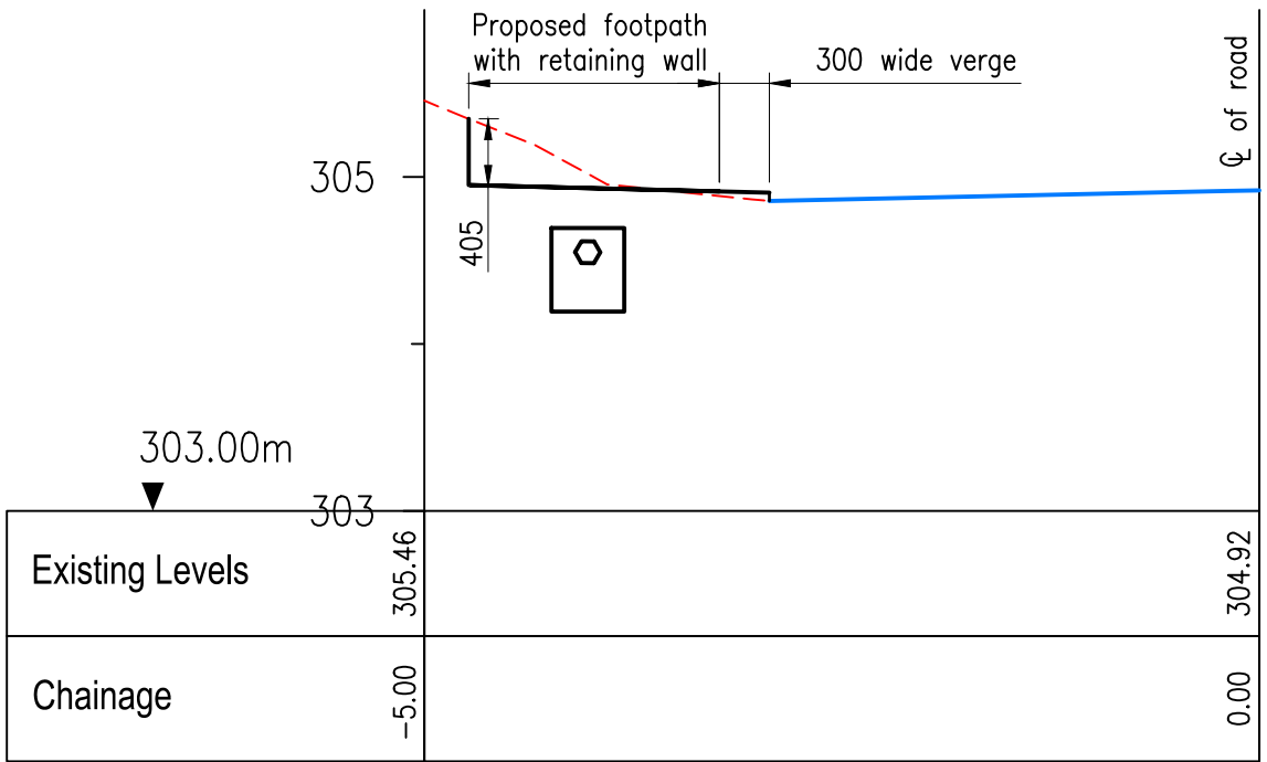
SECTION 6 - Ch83 Scale 1:50
