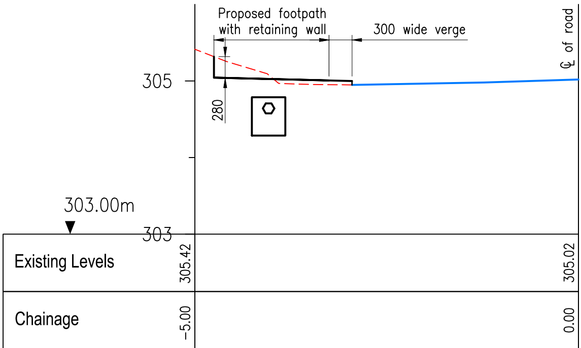
SECTION 4 - Ch45 Scale 1:50
